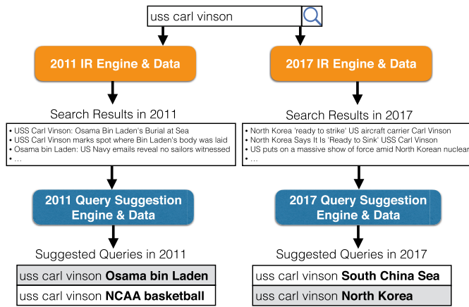
Figure 1: Example of search result volatility and its impact on an hypothetical query expansion techniques that exploits the retrieved results.
